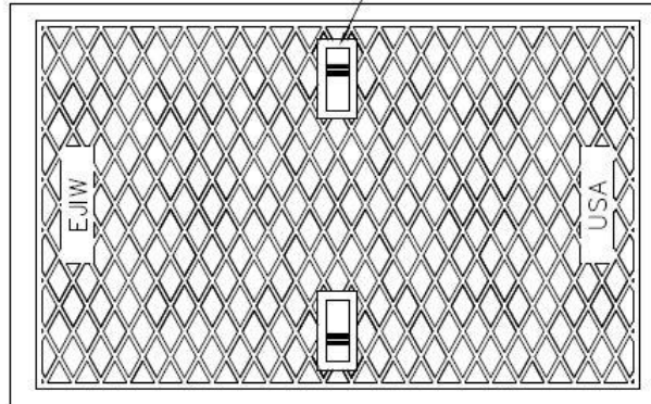
COVER TOP VIEW
