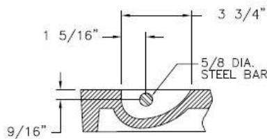
TYPE 4A PICKBAR DETAIL
